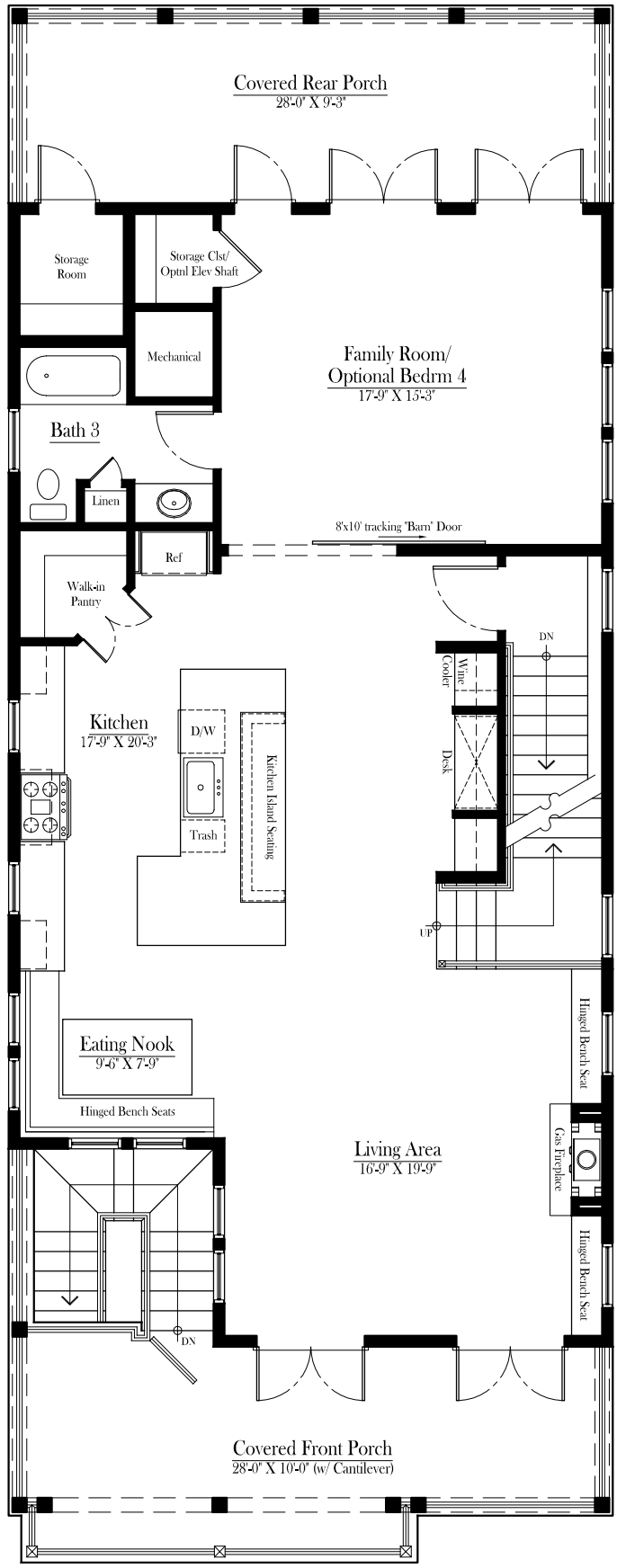
First Floor Plan Scale: 1/8"=1'-0"
